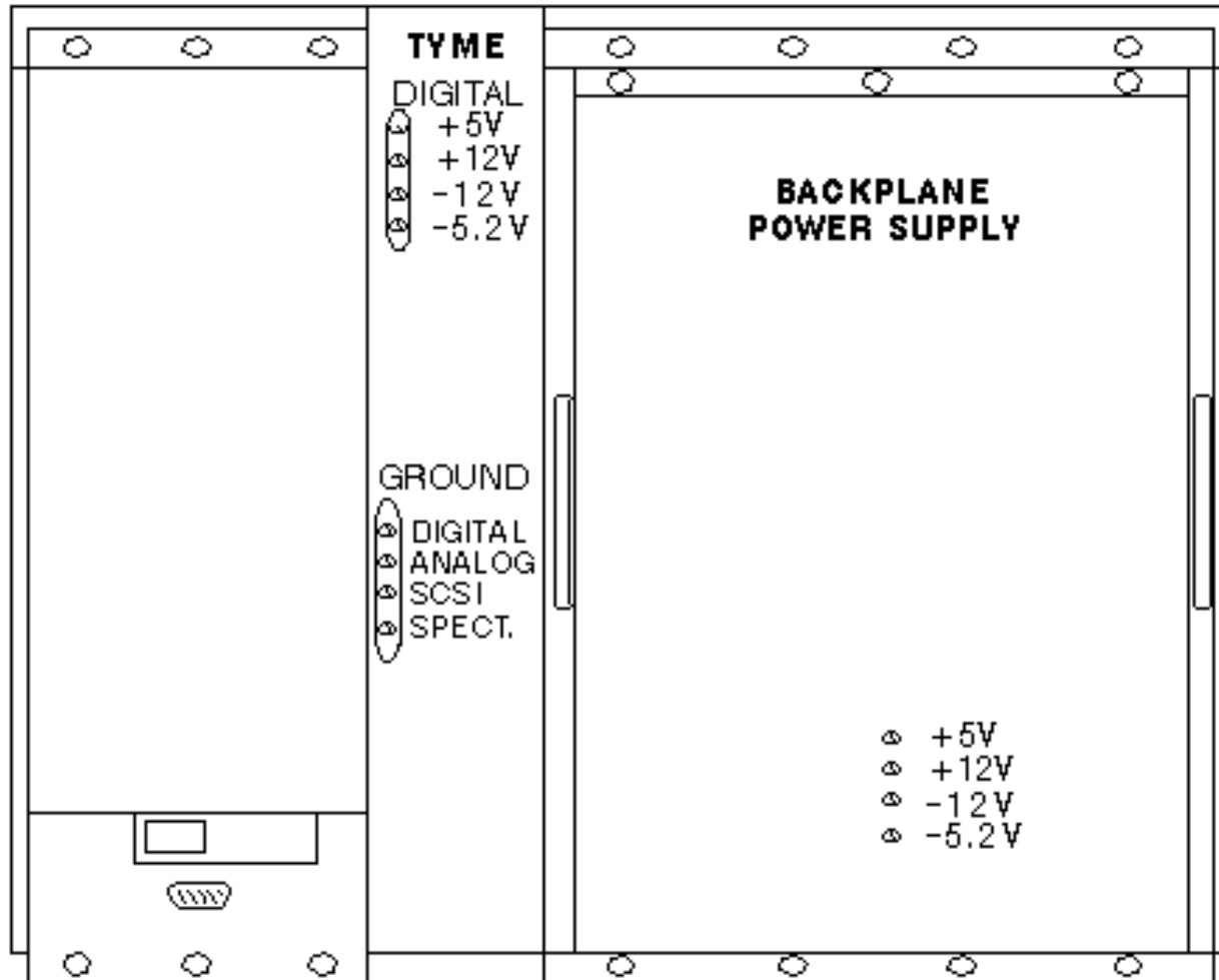
BACKPLANE TEST POINTS AND ADJUSTMENT LOCATIONS ILLUSTRATION L4759A
